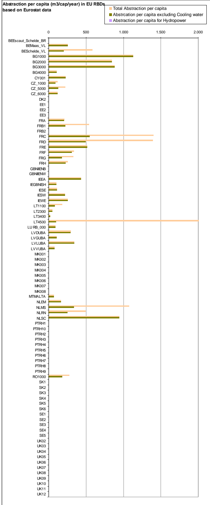
Figure 8.9 – Abstraction per capita (m 3 /cap/year) in EU RBDs, based on Eurostat data
