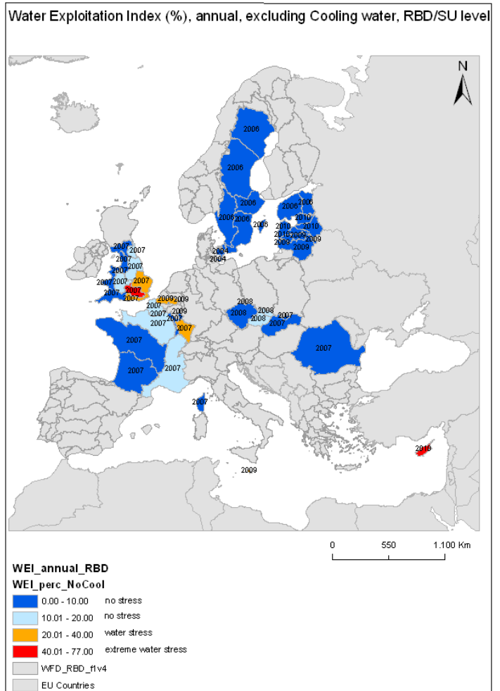
Map 8.9 – WEI annual at RBD/SU excluding Cooling water
