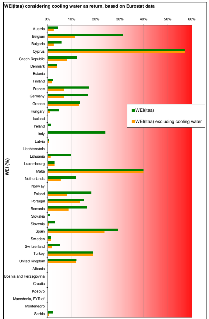
Figure 8.4 - WEI(ltaa) considering cooling water as return, based on Eurostat data
