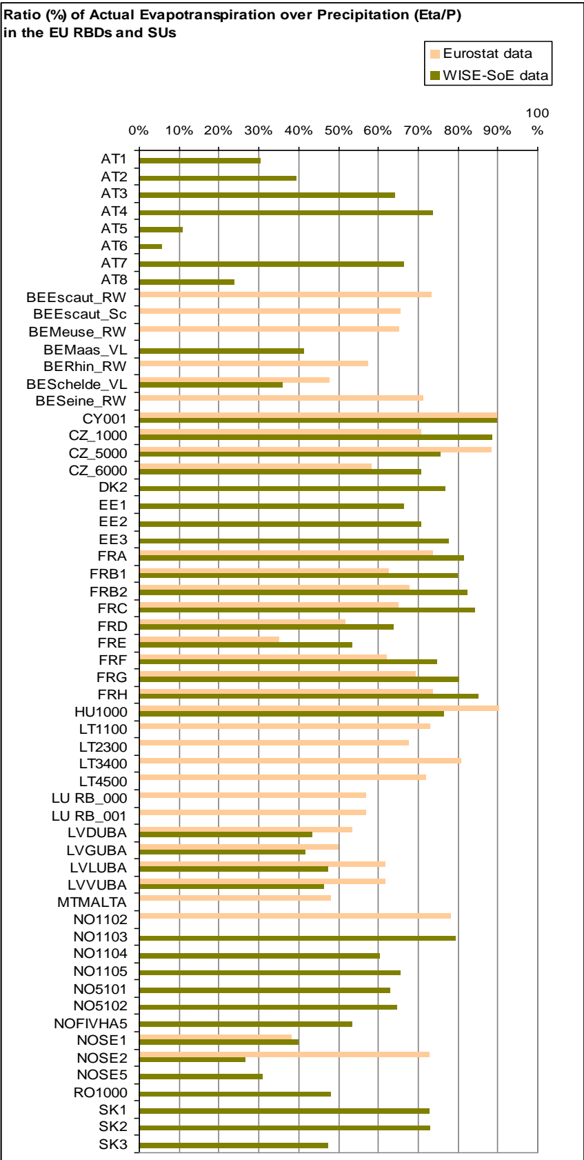
Figure 8.12 - Ratio (%) of Actual Evapotranspiration (ETa) over Precipitation (P) based on WISE-SoE and Eurostat data
