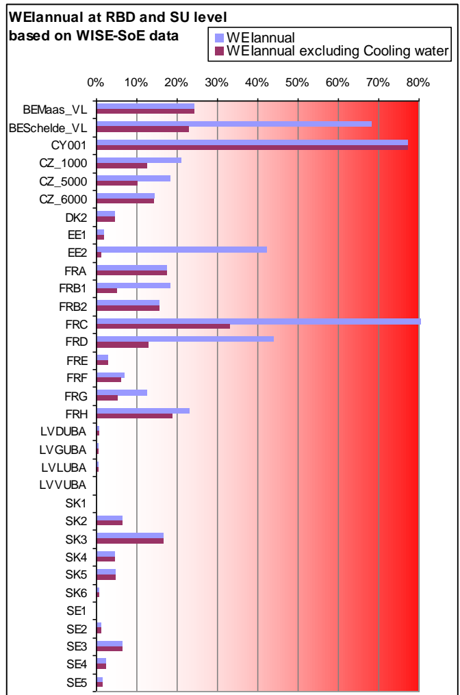
Figure 8.14 - WEIannual per RBD based on WISE-SoE data
