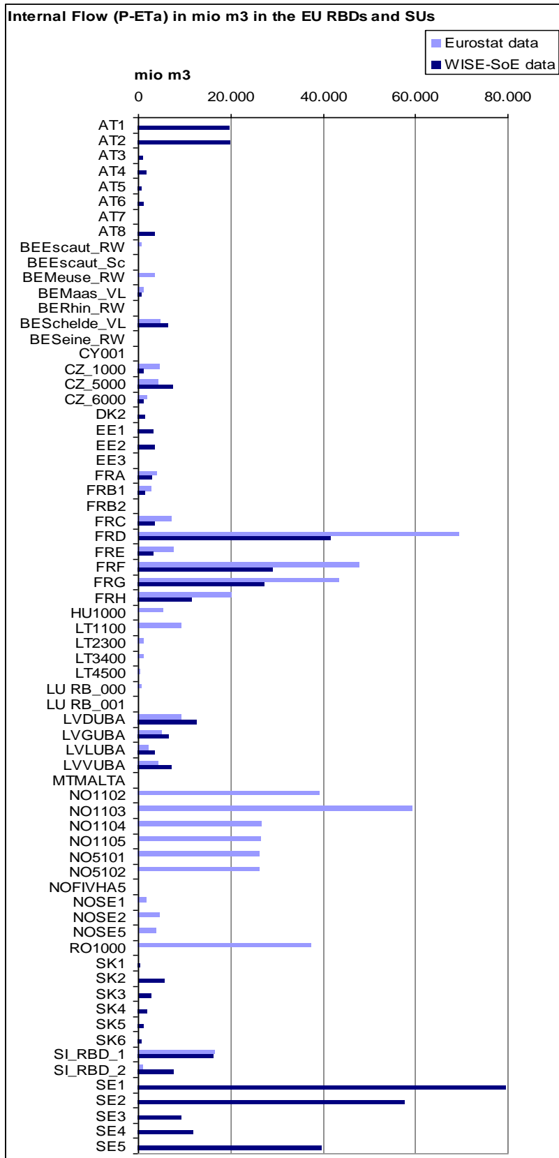
Figure 8.11 – Internal Flow (P-ETa) in mio m3 based on WISE-SoE and Eurostat data
