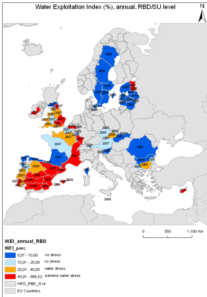
Map 8.8 – WEI annual at RBD/SU level
