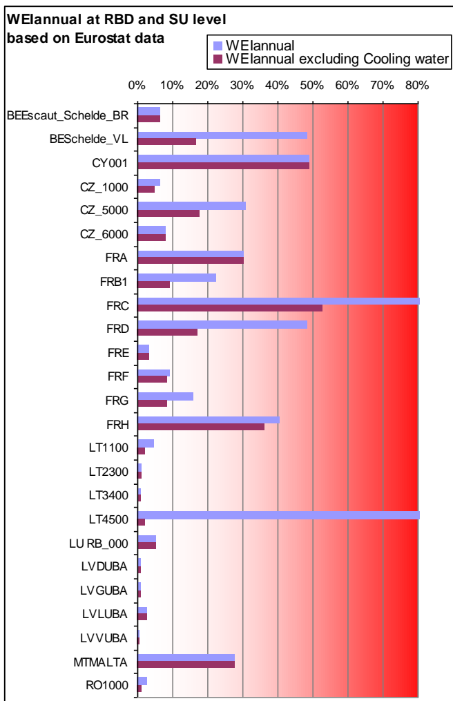
Figure 8.13 – WEIannual per RBD based on Eurostat data
